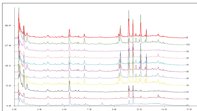
Figure 3: Chromatograms of the fingerprints of the 10 samples. The chromatograms of the 10 samples were obtained at 285 nm. Twenty-seven peaks were identified as the characteristic peaks
