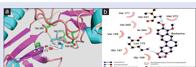
Figure 4: Docking berberine into the ATP binding site of myosin light-chain kinase. (a) The binding mode of berberine to the ATP binding site of myosin light-chain kinase. Berberine forms two hydrogen bonds with Lys173 and Val221. The negatively charged side chains of Asp285 and Glu269 may stabilize the binding of the positively charged berberine via electrostatic attraction. (b) Illustration of interaction between berberine and myosin light-chain kinase. The binding of berberine to the myosin light-chain kinase is driven by the hydrophobic interaction with residues such as Ala171, Met272, Val202, Ile284, Val158, in addition to two hydrogen bonds
