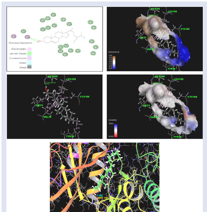
Figure 4: Photographs shows the docking analysis of ERK-2 with \beta -sitosterol visualised by Maestro 10.3 visualiser and Discovery studio 4.1 visualiser.
